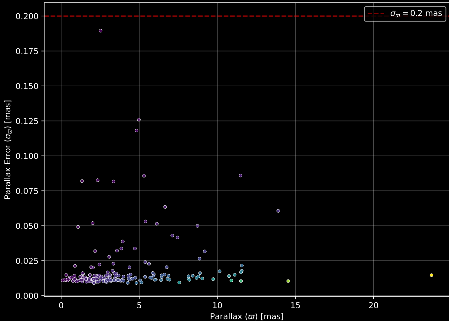
APOGEE DR17 Field: [092+65_MGA] Parallax Quality (n= 196)
