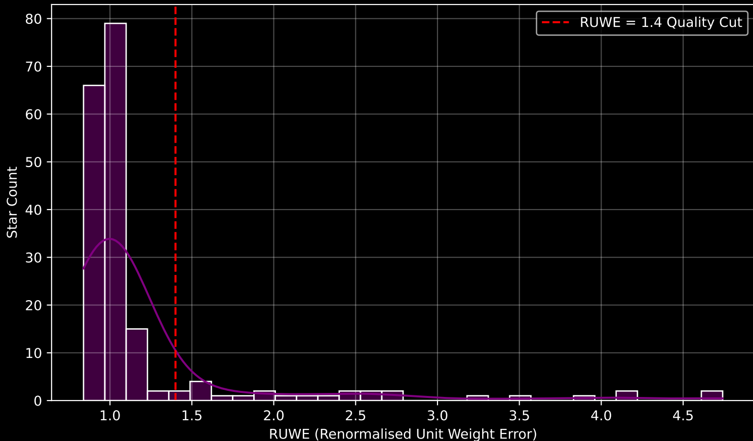
GAPOGEE DR17 Field [092+65_MGA] RUWE Distribution (n= 188)
