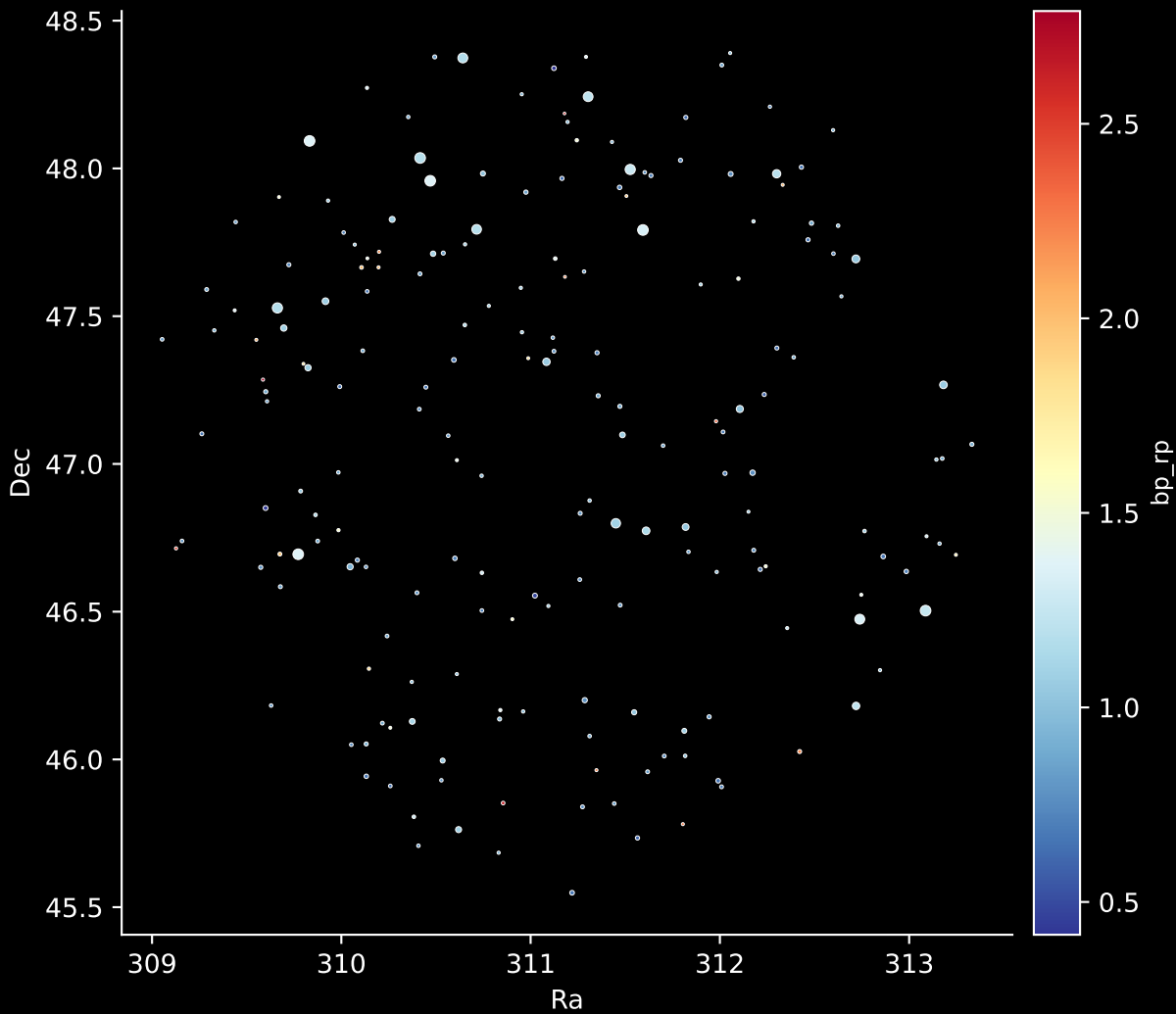
APOGEE DR17 Field: [092+65_MGA] Stars: 196
