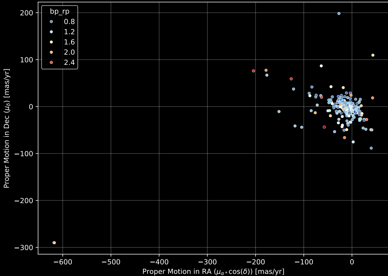
APOGEE DR17 Field: [092+65_MGA] Proper Motion Diagram (n= 196)
