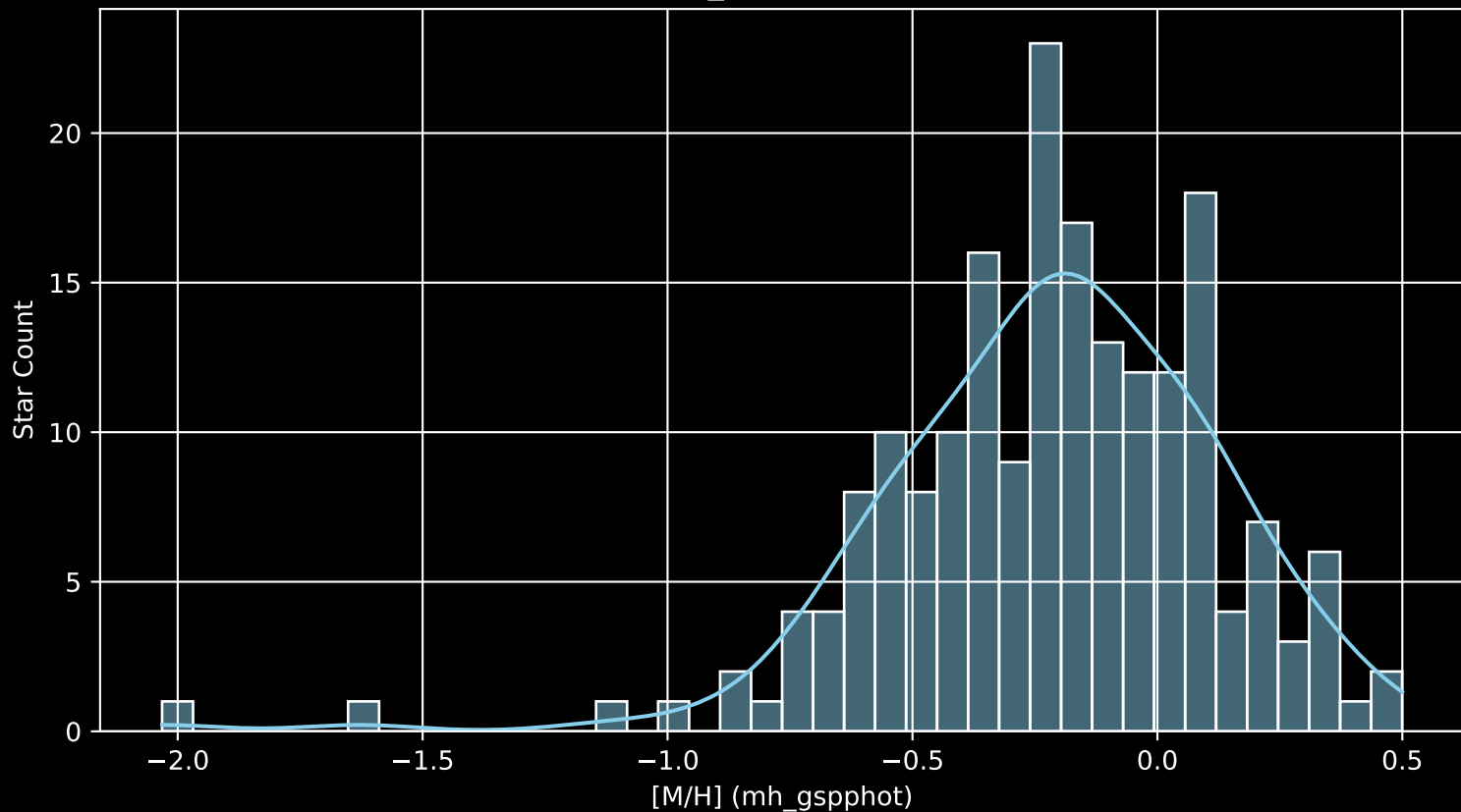
APOGEE DR17 Field: [092+65_MGA [M/H] (mh_gspphot) (n= 194)
