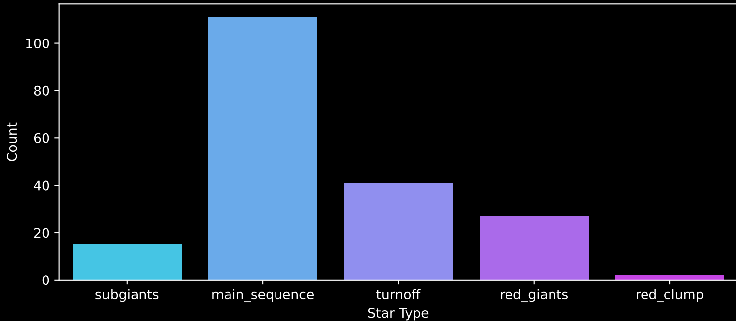
APOGEE DR17 Field: [092+65_MGA] Count plot of Star Type
